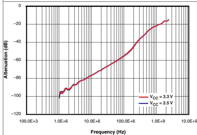
Figure 3. Crosstalk vs Frequency
