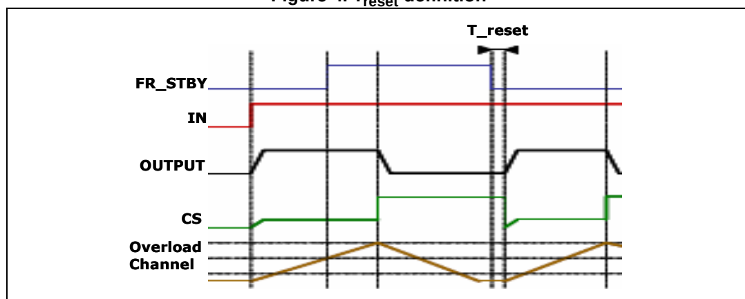
Figure 4. T_{reset} definition
