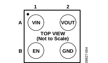
Figure 5. 4-Ball WLCSP Pin Configuration
