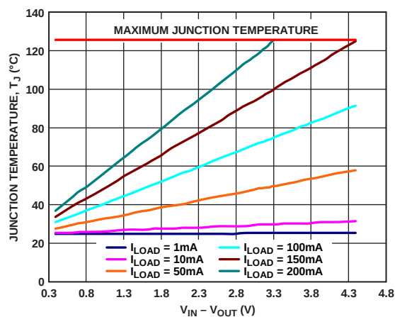
Figure 39. WLCSP 500 mm² of PCB Copper, T_A = 25^\circ\text{C}
