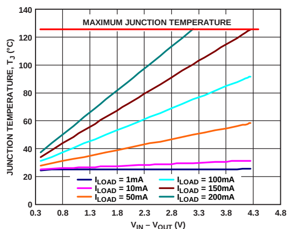
Figure 40. WLCSP 100 mm² of PCB Copper, T_A = 25^\circ\text{C}
