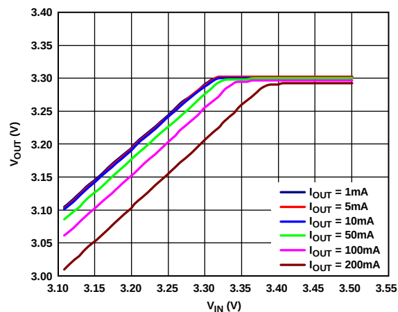
Figure 15. Output Voltage vs. Input Voltage (in Dropout)
