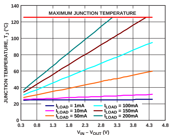
Figure 41. WLCSP 50 mm² of PCB Copper, T_A = 25^\circ\text{C}
