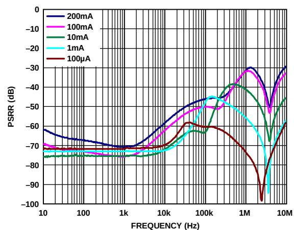
Figure 17. Power Supply Rejection Ratio vs. Frequency, V_{OUT} = 1.2\text{ V} , V_{IN} = 2.2\text{ V}
