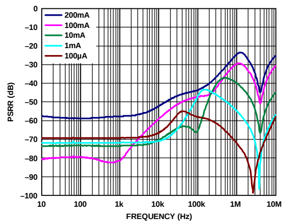
Figure 18. Power Supply Rejection Ratio vs. Frequency, V_{OUT} = 2.8\text{ V} , V_{IN} = 3.3\text{ V}
