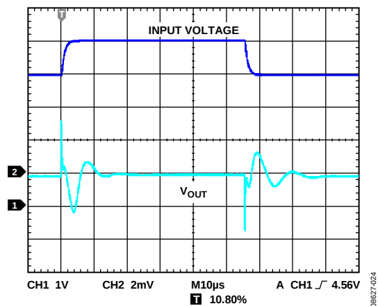
Figure 26. Line Transient Response, C_{IN}, C_{OUT} = 1 \mu F, I_{LOAD} = 1 mA
