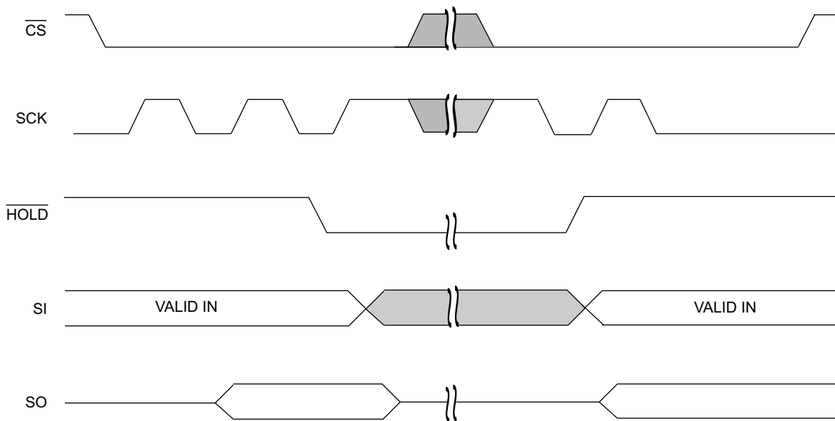
Figure 13. \overline{\text{HOLD}} Operation [2]
