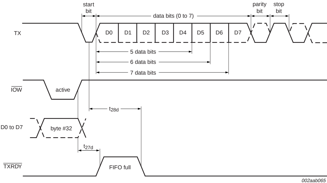
Fig 24. Transmit ready timing in FIFO mode (DMA mode '1')
