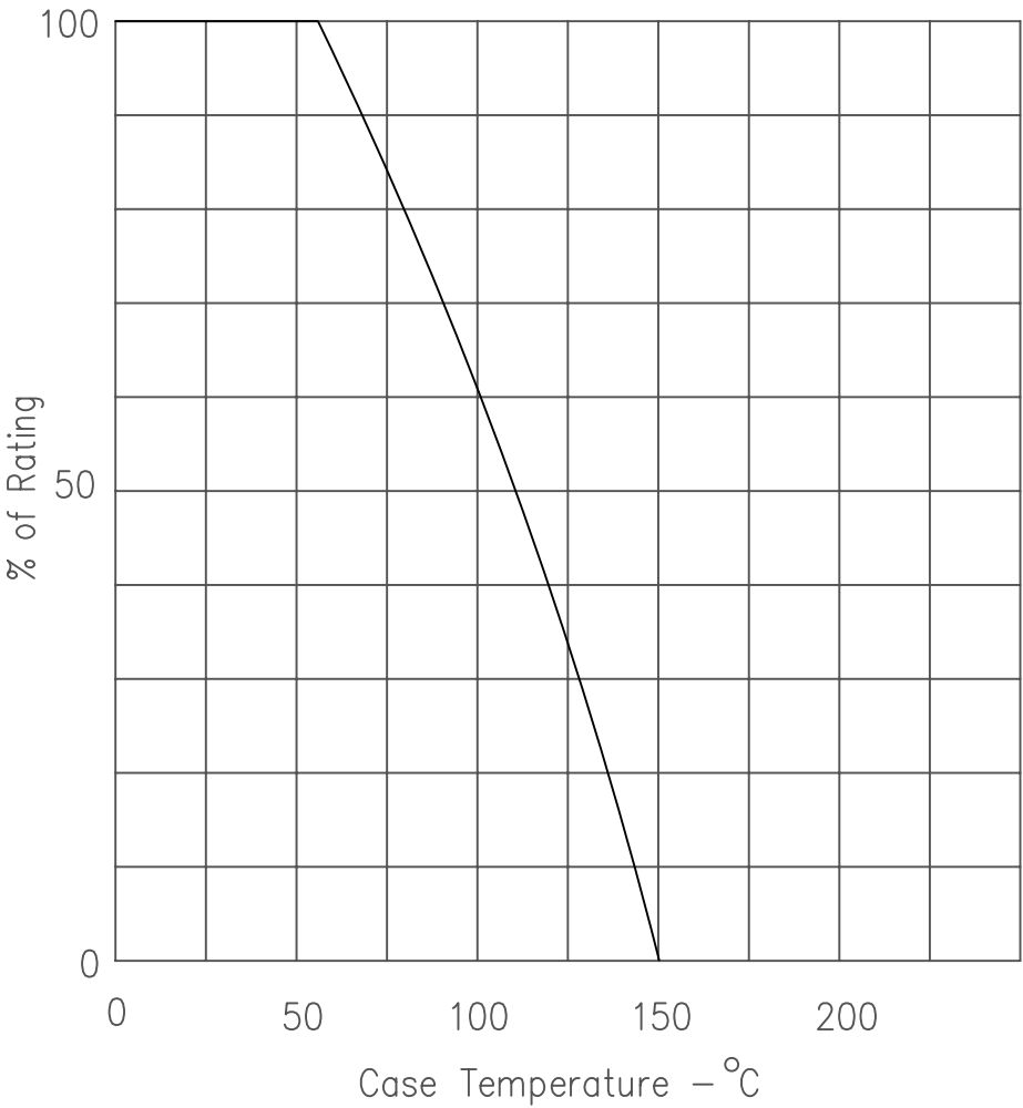
Figure 3 Current Derating
