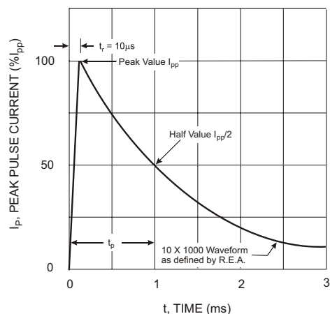
Fig. 4 Pulse Waveform
