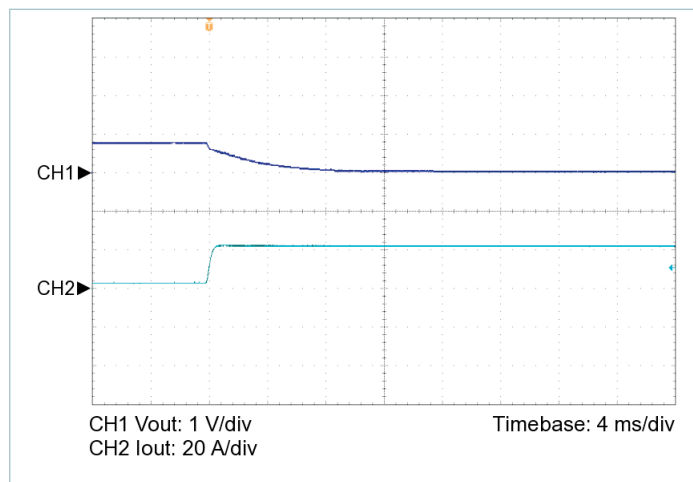
Figure 8 — 10% to 100% load transient response, V_{IN} = 24\text{ V} , nominal trim, C_{OUT\_EXT} = 680\text{ }\mu\text{F}
