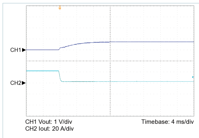
Figure 7 — 100% to 10% load transient response, V_{IN} = 24\text{ V} , nominal trim, C_{OUT\_EXT} = 680\text{ }\mu\text{F}
