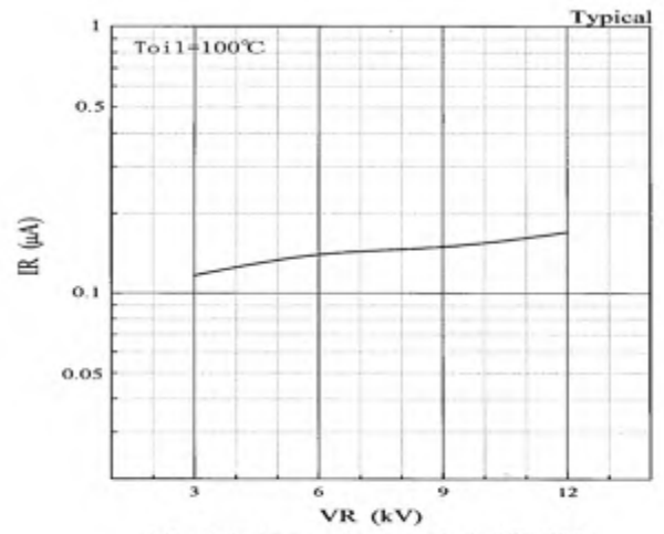
Fig. 2 Reverse characteristic [VR-IR]
