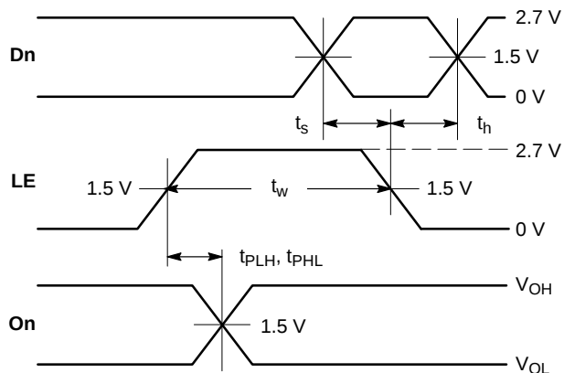
WAVEFORM 3 – LE to On PROPAGATION DELAYS, LE MINIMUM
