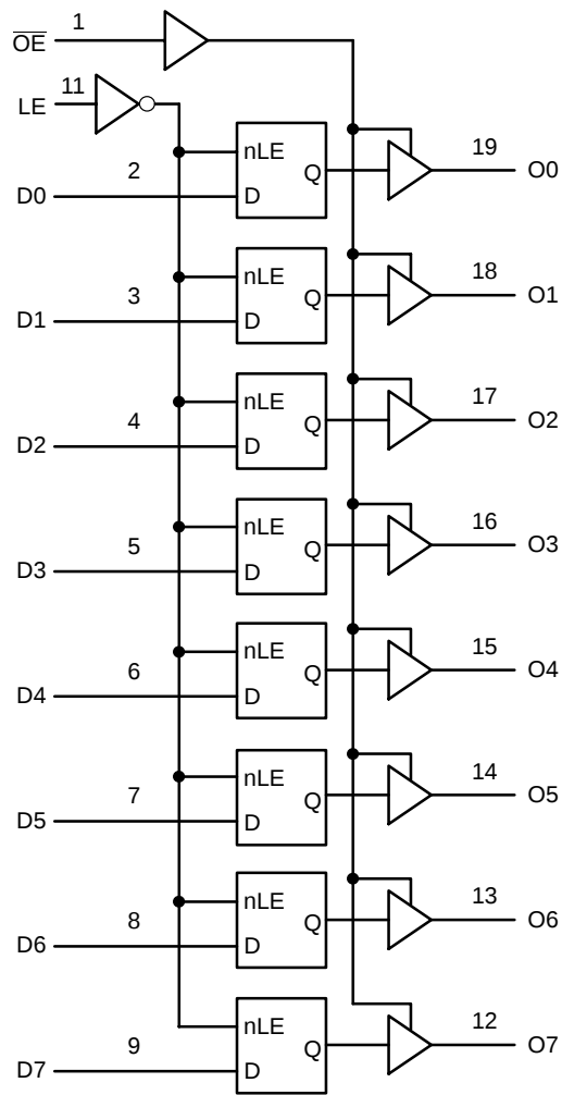
Figure 2. Logic Diagram
