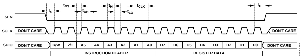
Figure 52. 1-Byte Serial Register Write in MSB-First Mode
