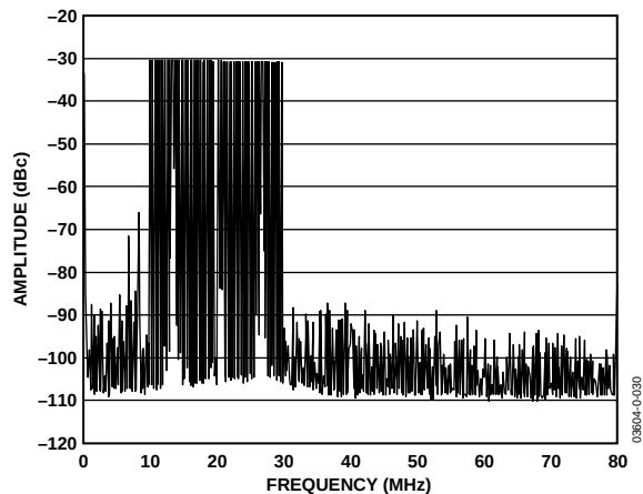
Figure 33. AD9863 Tx Path FFT of OFDM Signal in Figure 28 with 2x Interpolation
