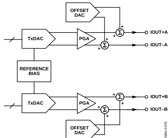
Figure 50. TxDAC Output Structure Block Diagram
