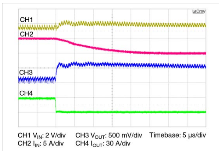
Figure 12 — 30 A – 0 A transient response: C_{IN} = 330 \mu F , I_{IN} measured prior to C_{IN} , no external C_{OUT}
