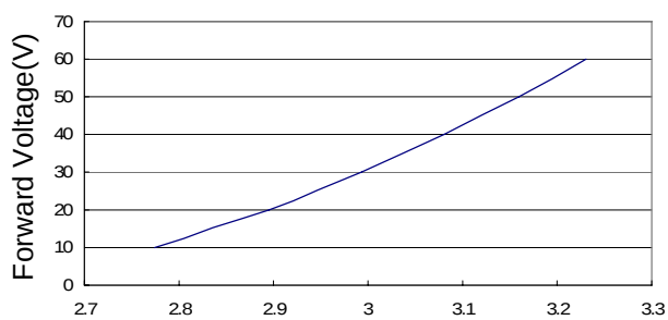
Fig.1 Forward current vs. Forward Voltage
