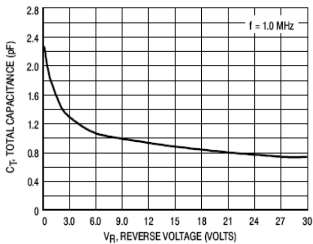
Figure 1. Total Capacitance
