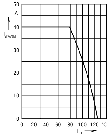
Fig. 7 Max. forward current versus heatsink temperature
