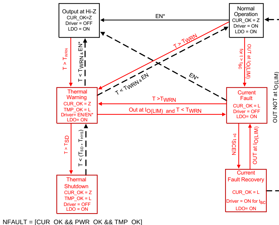
Figure 10. Device State Diagram
