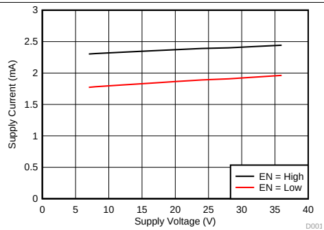
Figure 1. Supply Current vs Supply Voltage
