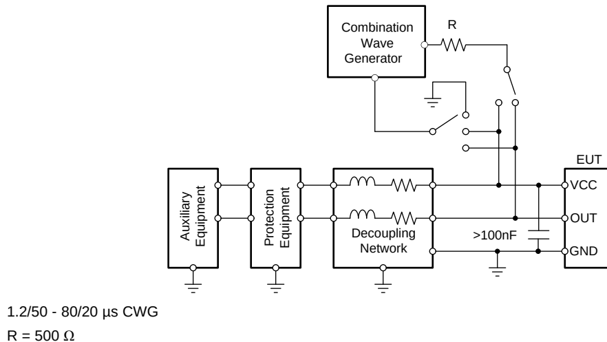
Figure 13. Surge Test Setup
