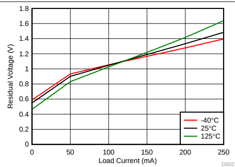
Figure 2. Residual Voltage vs Load Current: High Side
