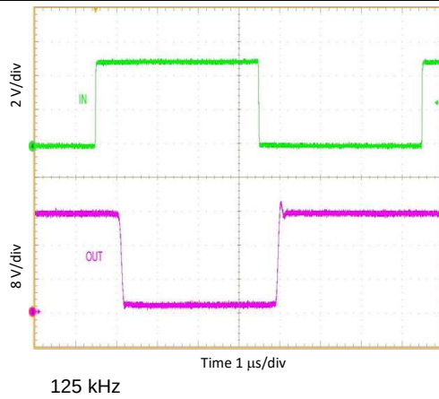
Figure 17. OUT in Push-Pull Mode
