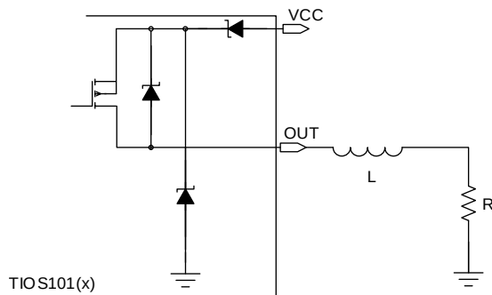
Figure 15. PNP Mode
