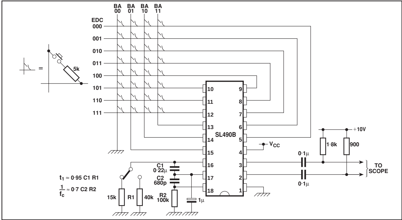
Fig. 4 Test circuit
