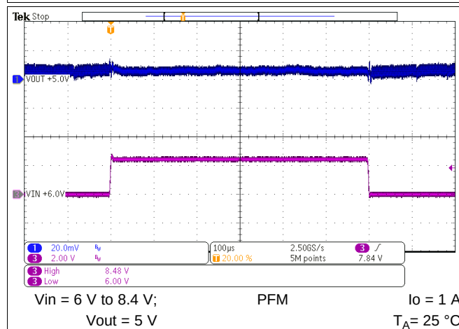
Figure 54. Line Transient Response
