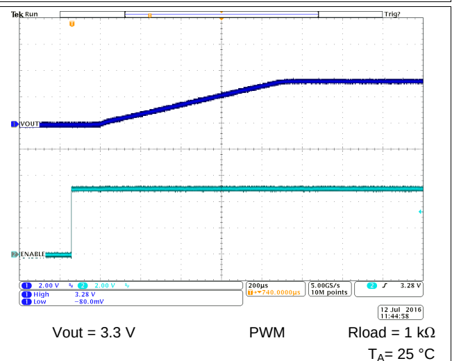
Figure 49. Start-Up Timing
