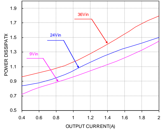
Full load input characteristics at room temperature.
