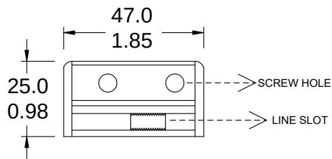
Side View2
