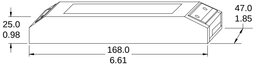
Side View1
