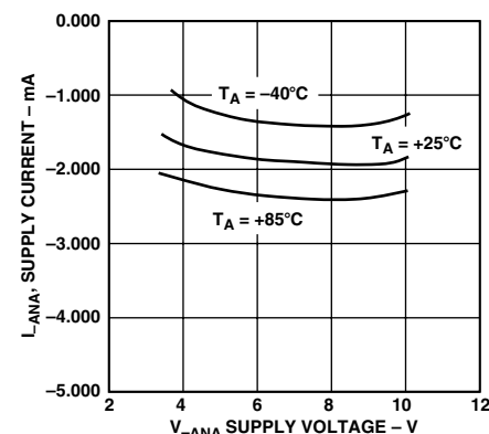
Figure 9. I_{-ANA} : Analog Supply Current/Comparator vs. Supply Voltage
