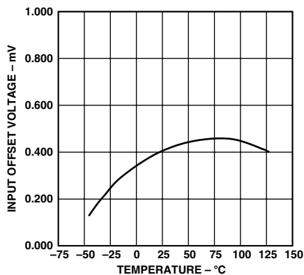
Figure 1. Input Offset Voltage vs. Temperature
