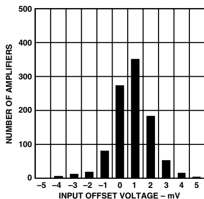
Figure 4. Input Offset Voltage
