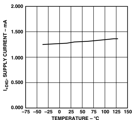
Figure 13. I_{+DIG} : Digital Supply Current/Comparator vs. Temperature
