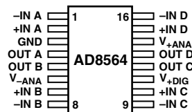
16-Lead TSSOP (RU-Suffix) RU-16
