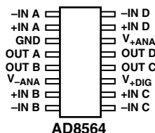
16-Lead Narrow Body SO (S Suffix) R-16A
