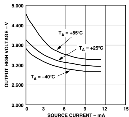
Figure 6. Output High Voltage, V_{OH} vs. Source Current
