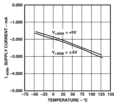
Figure 12. I_{-ANA} : Analog Supply Current/Comparator vs. Temperature
