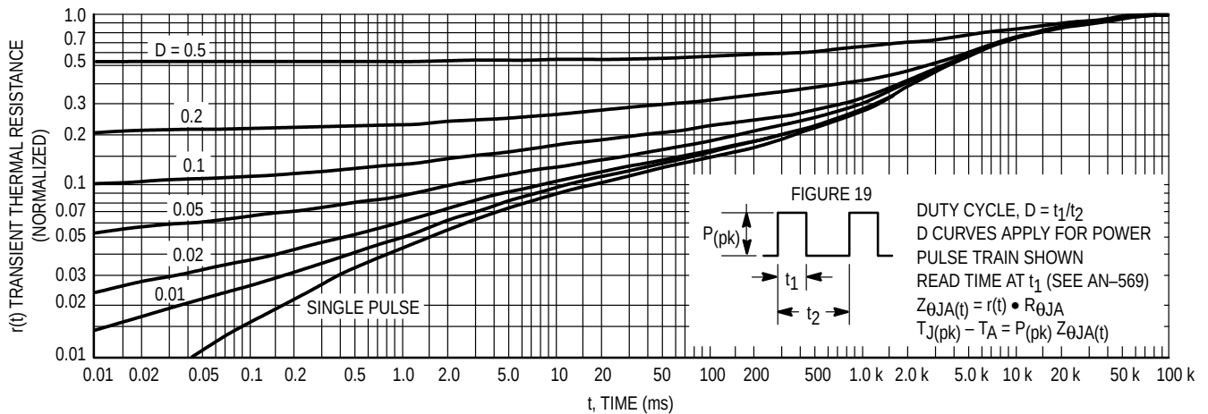
Figure 14. Thermal Response
