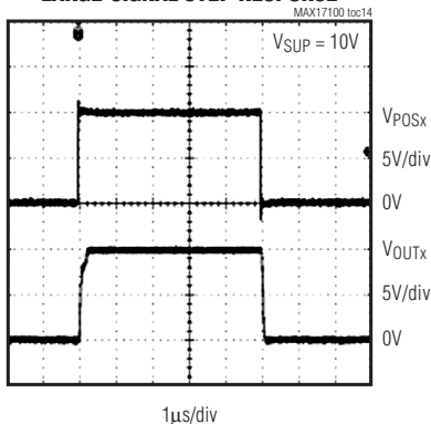
OPERATIONAL AMPLIFIER LARGE-SIGNAL STEP RESPONSE
