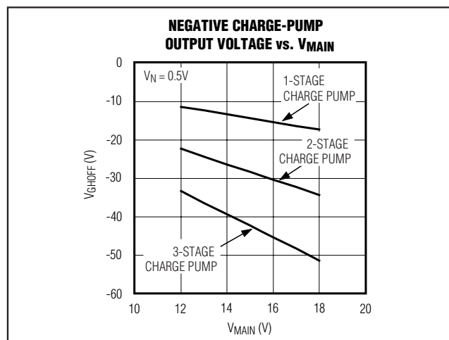
Figure 12. Negative Charge-Pump Output Voltage vs. V_{MAIN}
