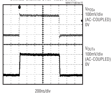
OPERATIONAL AMPLIFIER SMALL-SIGNAL STEP RESPONSE
