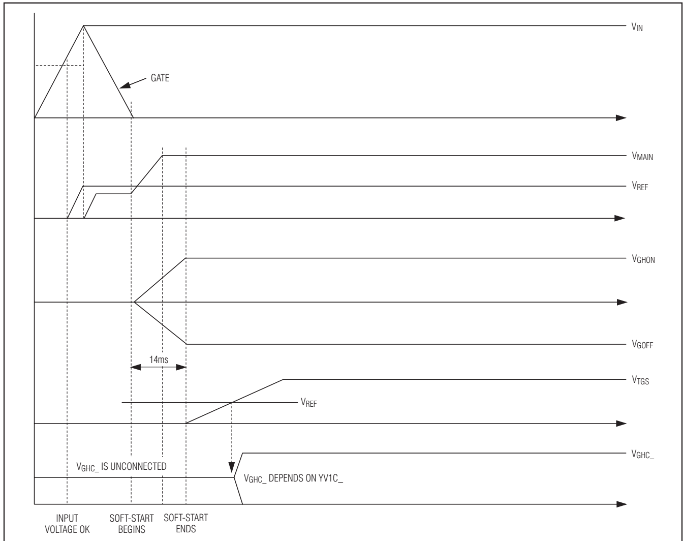
Figure 7. Power-Up Sequence
