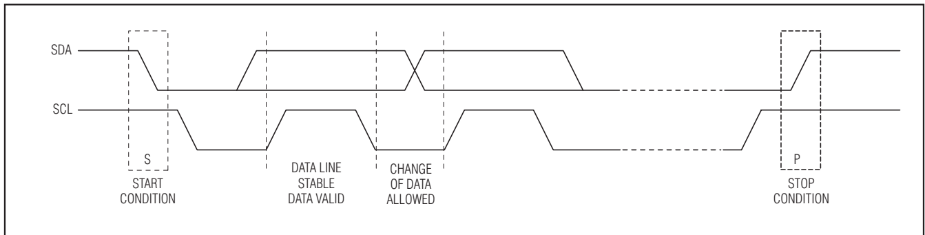
Figure 13. Serial Bus START, STOP, and Data Change Conditions
