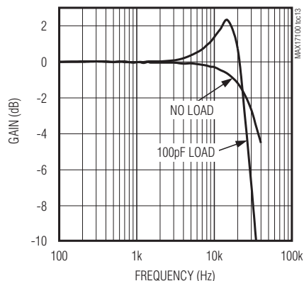
OPERATION AMPLIFIER FREQUENCY RESPONSE
