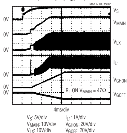
POWER-UP SEQUENCE
