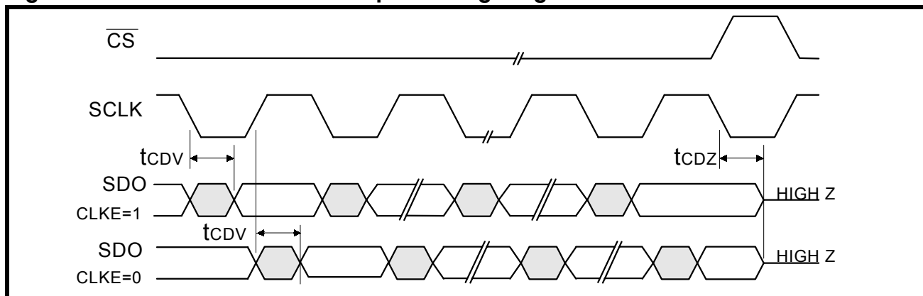
Figure 17: LXT318 Serial Data Output Timing Diagram
