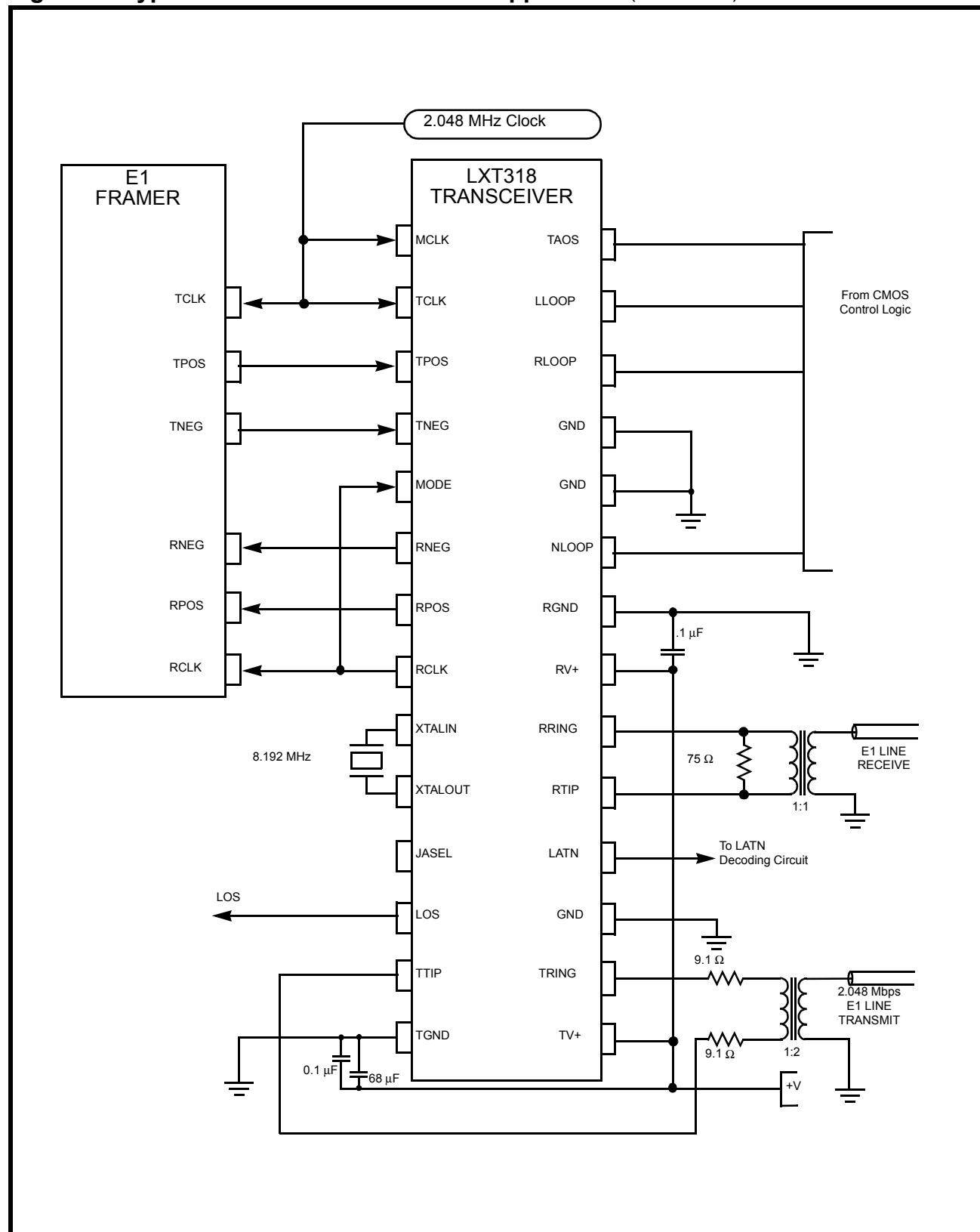
Figure 13: Typical LXT318 Hardware Mode Application (75 \Omega Coax)
