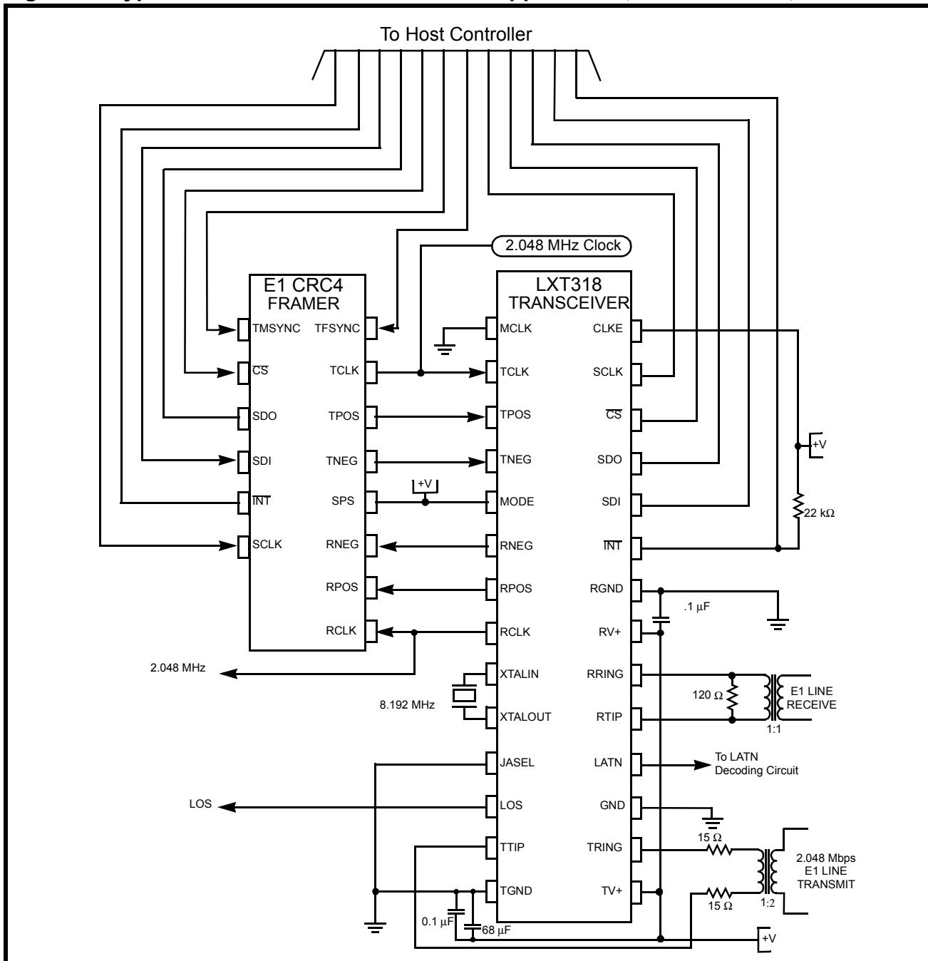
Figure 11: Typical LXT318 Host Mode E1/NTU Application (120 \Omega Twisted Pair)
