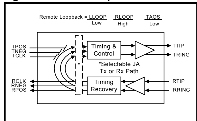
Figure 9: Remote Loopback
