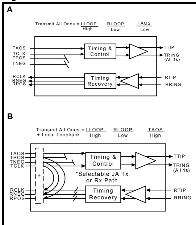
Figure 8: Local Loopback
