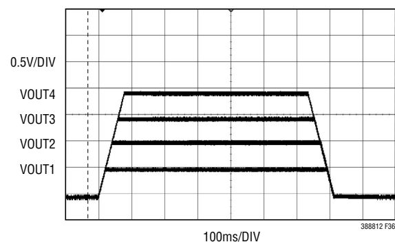
Figure 36. LTC3888-1 Time-Based Coincident Supply Ramping
