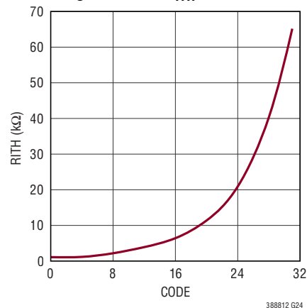
Programmable R ITH
