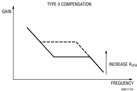
Figure 29. R_{ITH} Adjust
