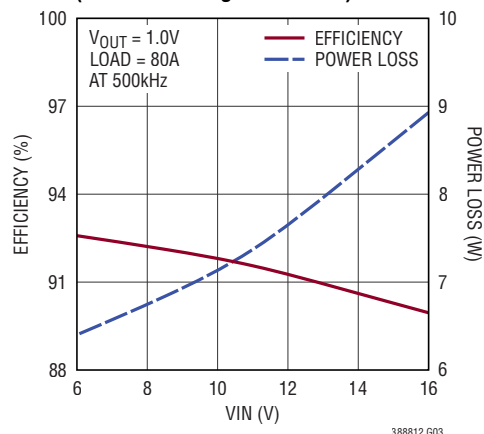
Efficiency and Power Loss vs Input Voltage (4-Phase Using TDA21470)
