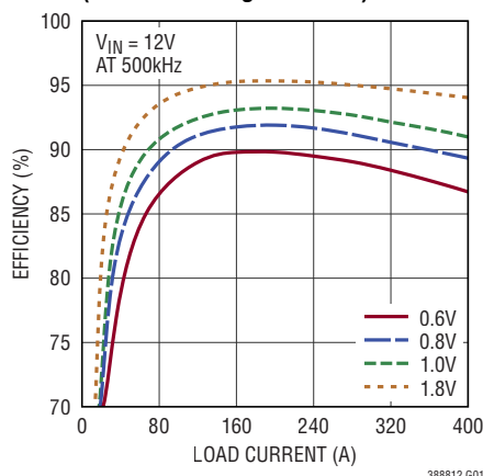
Efficiency vs Load Current (8-Phase Using LTC7051)
