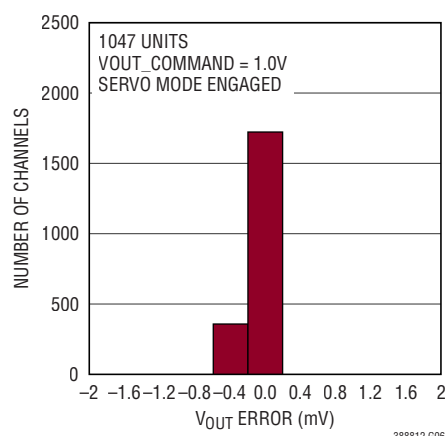
Typical Output Voltage Distribution at 25°C with Servo
