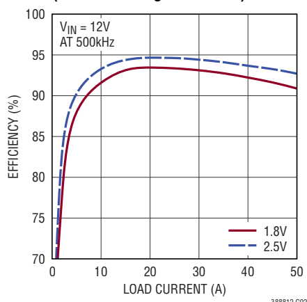
Efficiency vs Load Current (1-Phase Using TDA21470)
