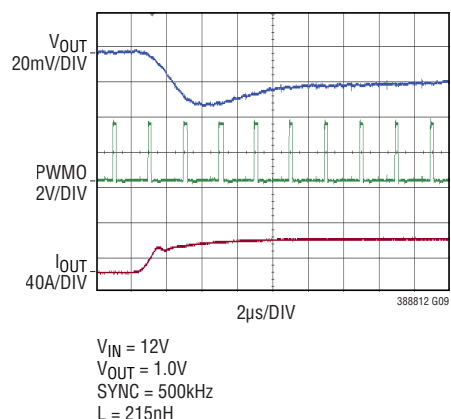
4-Phase Single Cycle Response (Using TDA21470 with C_{OUT} = 4mF )
