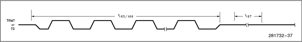
Figure 11-23. Jabber Timings
