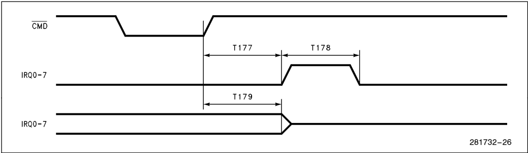
Figure 11-13. Interrupt Timing
