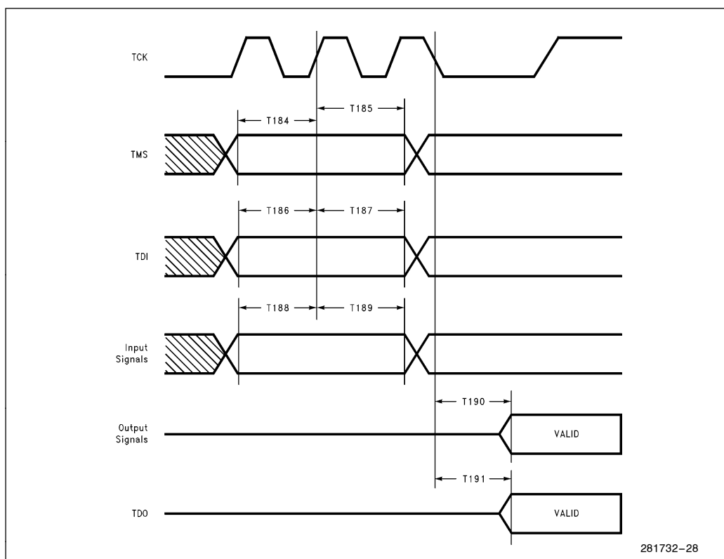
Figure 11-15. 82595FX JTAG Timing
