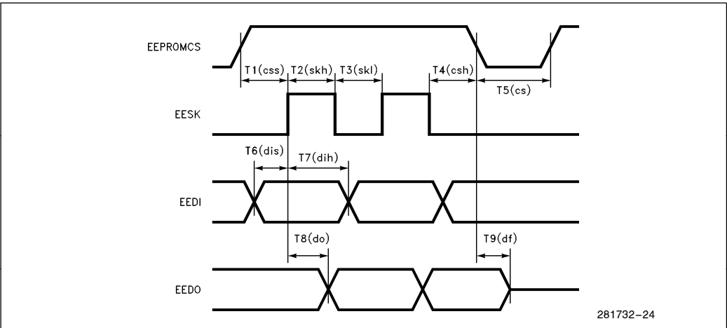
Figure 11-12. EEPROM Timings
