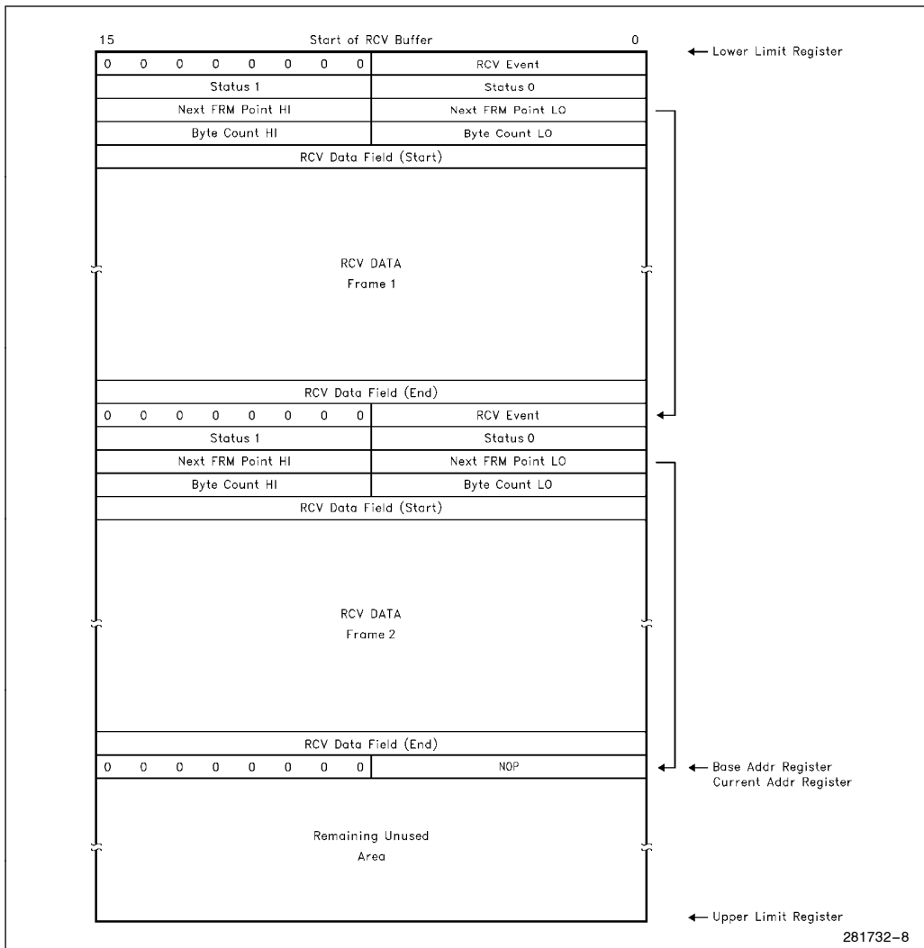
Figure 8-1. 82595FX RCV Memory Structure (16-Bit)
