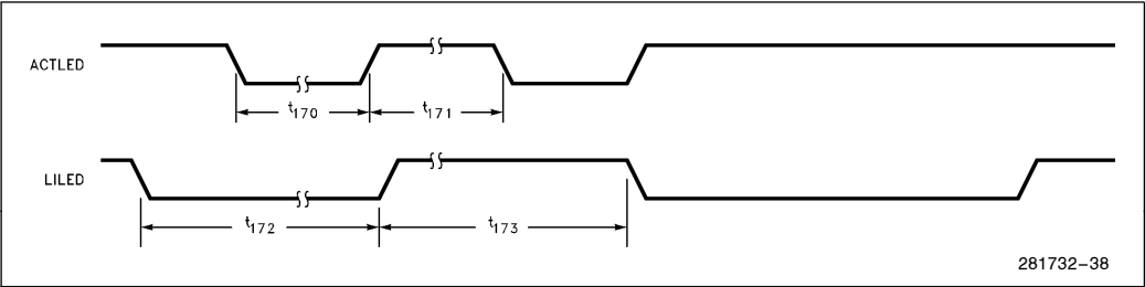
Figure 11-24. LED Timings
