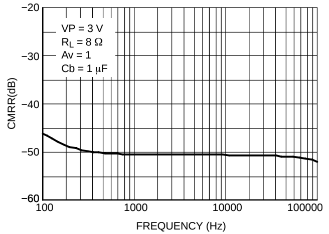
Figure 16. CMRR @ V_P = 3 \text{ V}
