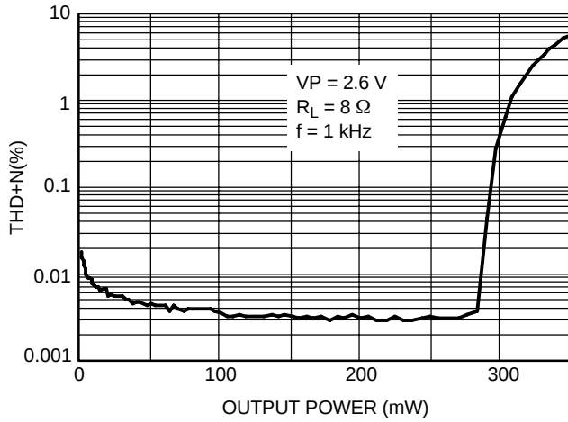
Figure 8. THDN versus Output Power
