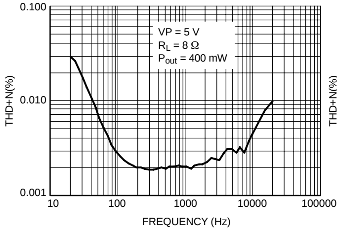
Figure 2. THDN versus Frequency
