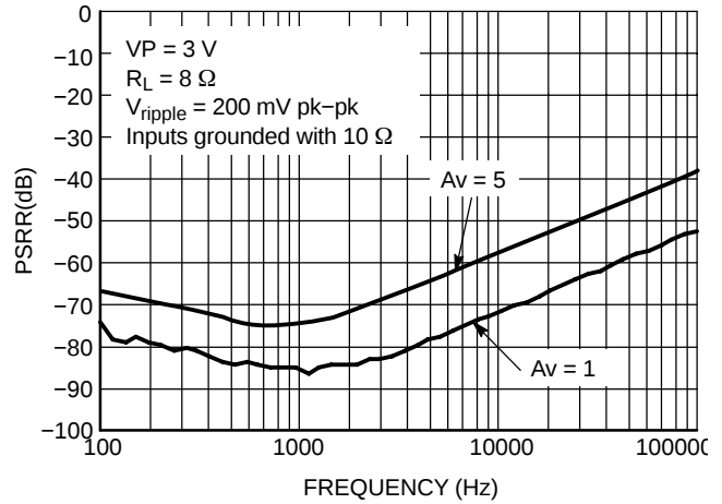
Figure 14. PSRR versus A_v @ V_P = 3 \text{ V}
