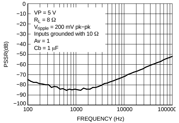
Figure 11. PSRR @ VP = 5 V
