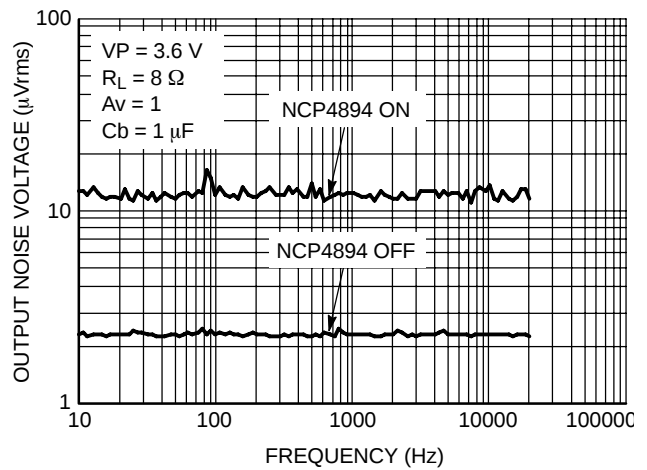
Figure 18. Noise Floor @ V_P = 3.6 \text{ V}
