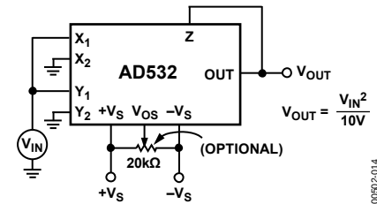
Figure 15. Squarer Connection
