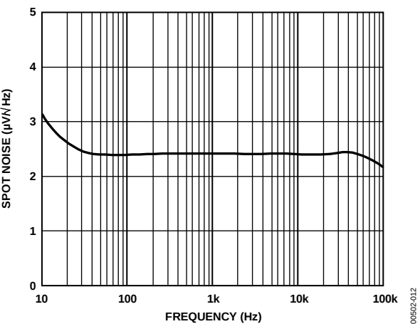
Figure 12. Spot Noise vs. Frequency
