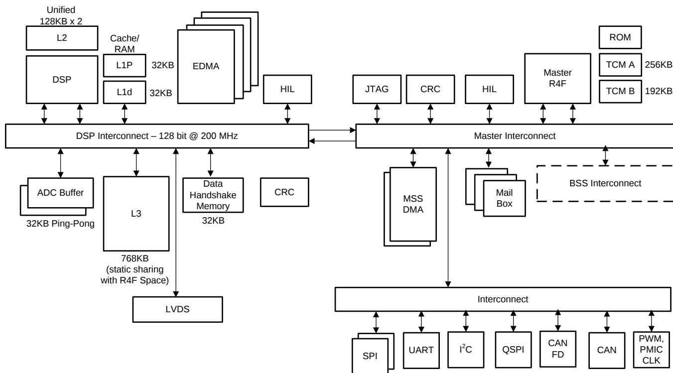
Figure 6-4. Processor Subsystem
