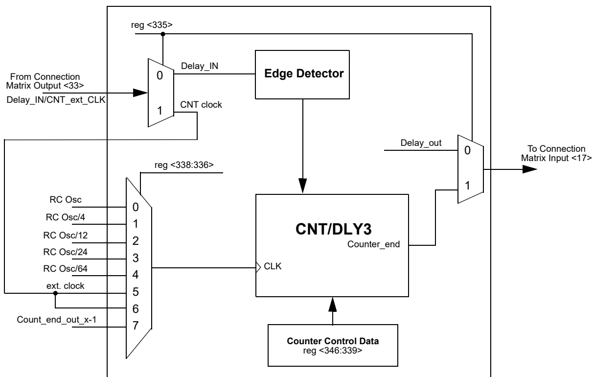
Figure 27. CNT/DLY3
