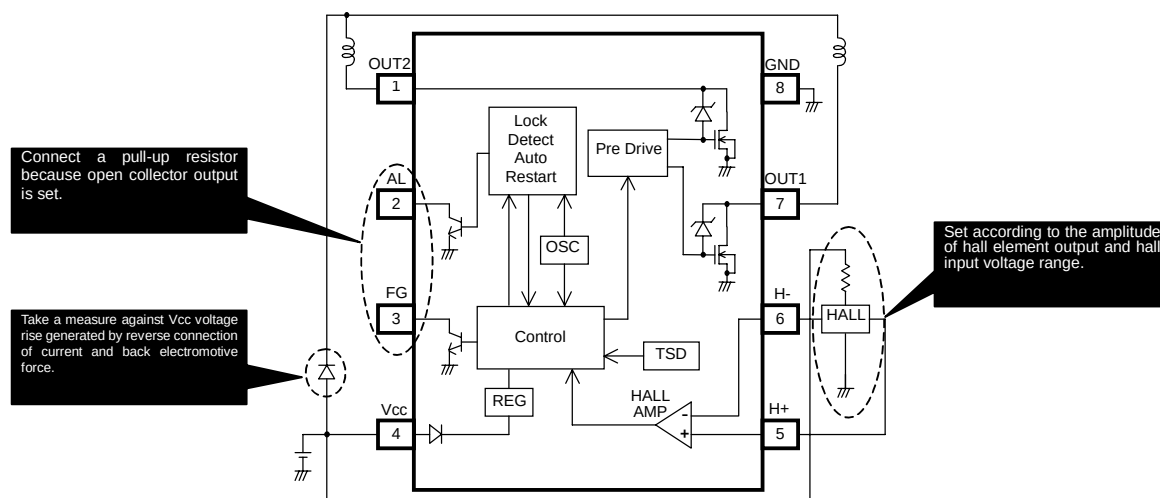
Fig.12 application circuit
