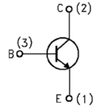
TO-92-FJ
