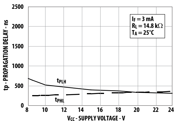
Figure 23 Typical Propagation Delay vs. Supply Voltage (ACPL-054L/W50L/K54L)
