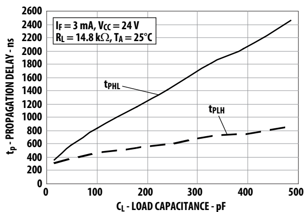
Figure 21 Typical Propagation Delay vs. Load Capacitance (ACPL-054L/W50L/K54L)
