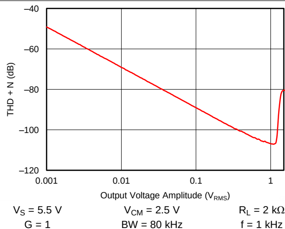
Figure 17. THD + N vs Amplitude
