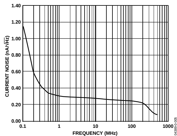
Figure 5. I_{OUT} Current Noise
