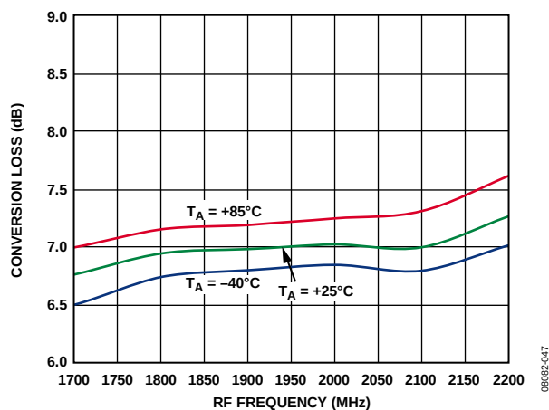
Figure 47. Power Conversion Loss vs. RF Frequency at 3.3 V, Upconversion
