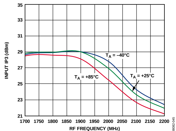
Figure 48. Input IP3 vs. RF Frequency at 3.3 V, Upconversion
