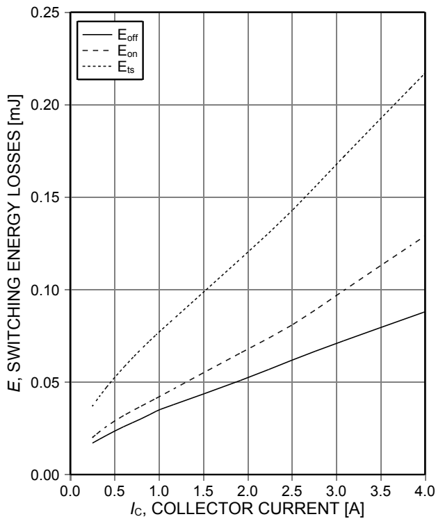
Figure 13. Typical switching energy losses as a function of collector current (inductive load, T_{vj}=175^{\circ}\text{C} , V_{CE}=400\text{V} , V_{GE}=15/0\text{V} , r_G=68\Omega , Dynamic test circuit in Figure E)
