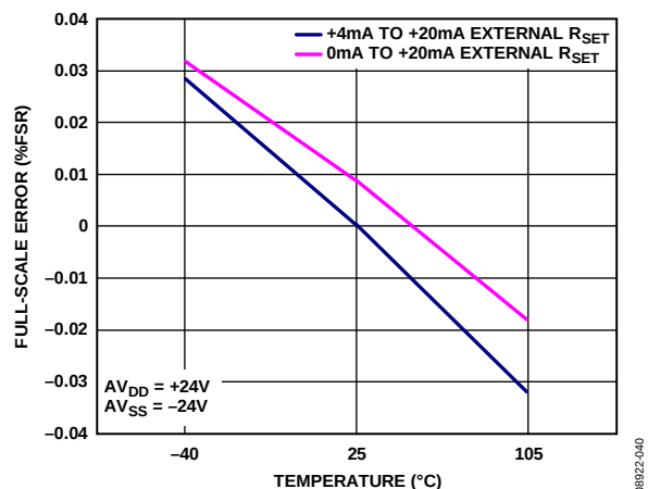
Figure 38. Full-Scale Error vs. Temperature, External R_{SET} Sense Resistor
