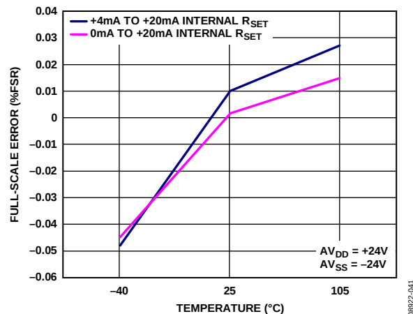
Figure 39. Full-Scale Error vs. Temperature, Internal R_{SET} Sense Resistor
