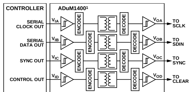
Figure 56. Isolated Interface
