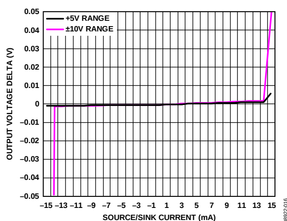
Figure 16. Source and Sink Capability of Output Amplifier
