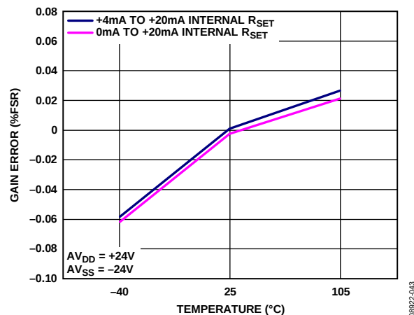
Figure 41. Gain Error vs. Temperature, Internal R_{SET} Sense Resistor
