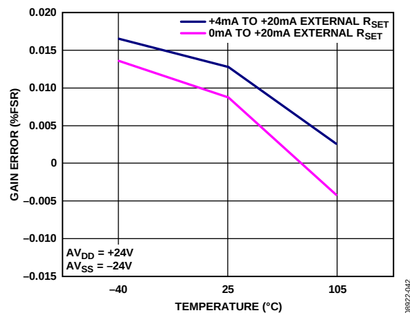
Figure 40. Gain Error vs. Temperature, External R_{SET} Sense Resistor
