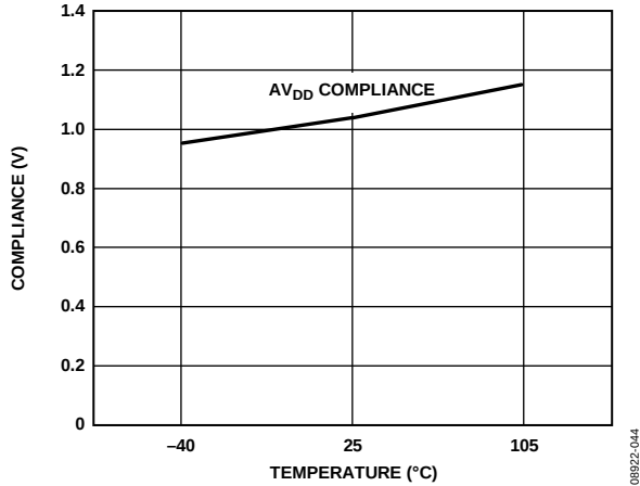
Figure 42. Output Compliance vs. Temperature Tested When I_{OUT} = 10.8 \text{ mA}
