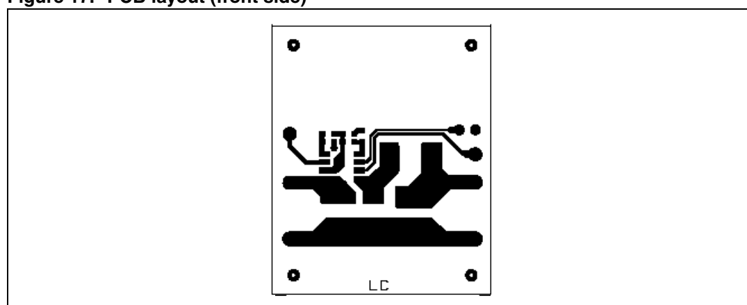
Figure 17. PCB layout (front side)
