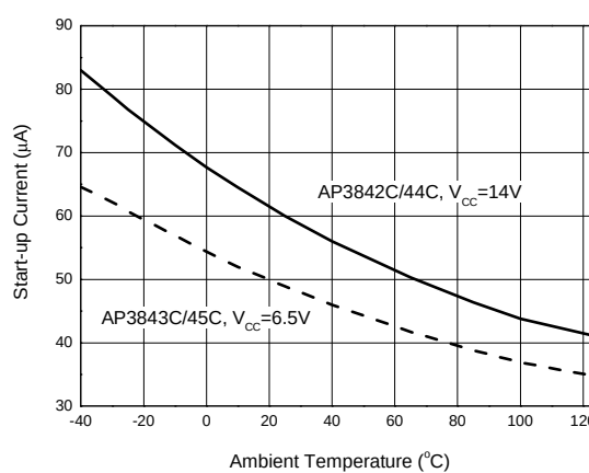
Figure 10. Start-up Current vs. Ambient Temperature
