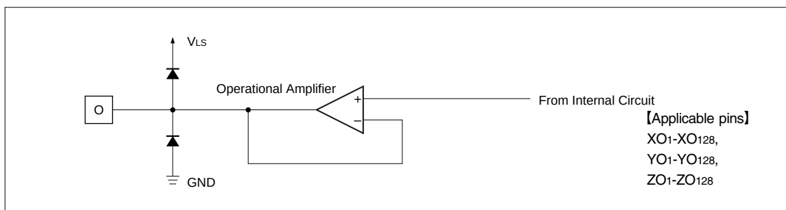
Fig. 4 Output Circuit
