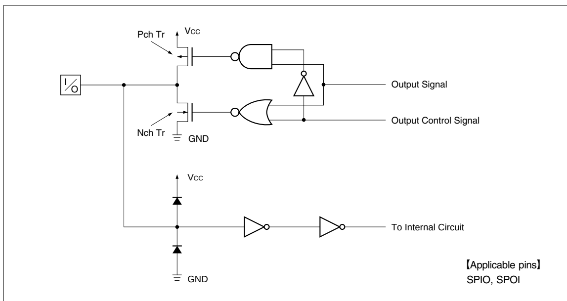
Fig. 3 Input/Output Circuit
