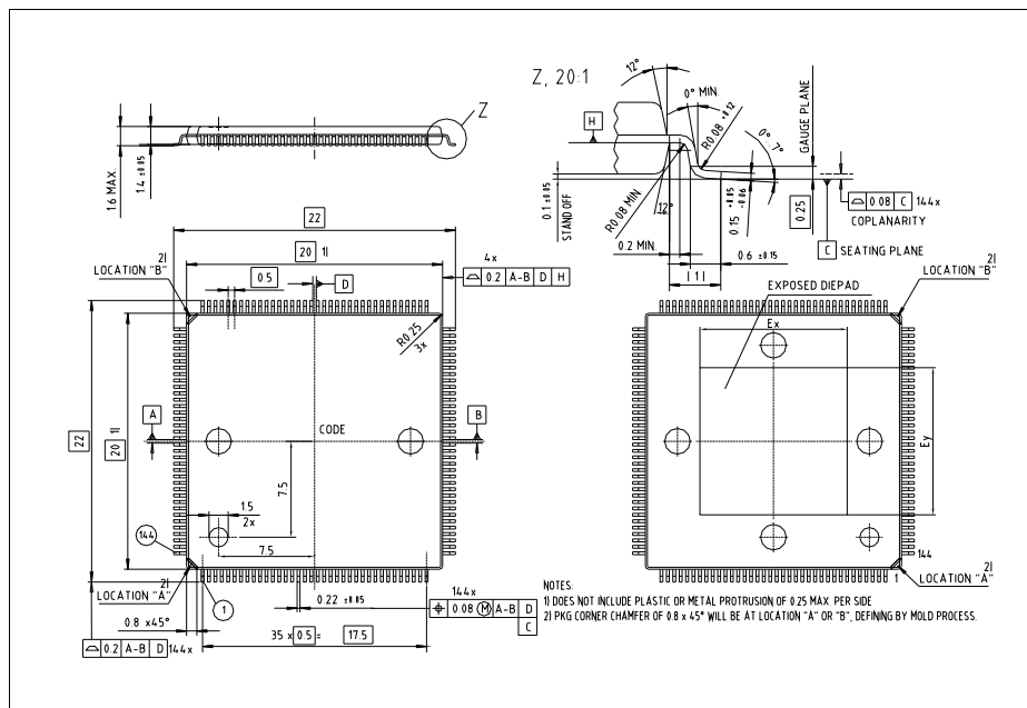
Figure 60 PG-LQFP-144-24 (Plastic Green Low Profile Quad Flat Package)
