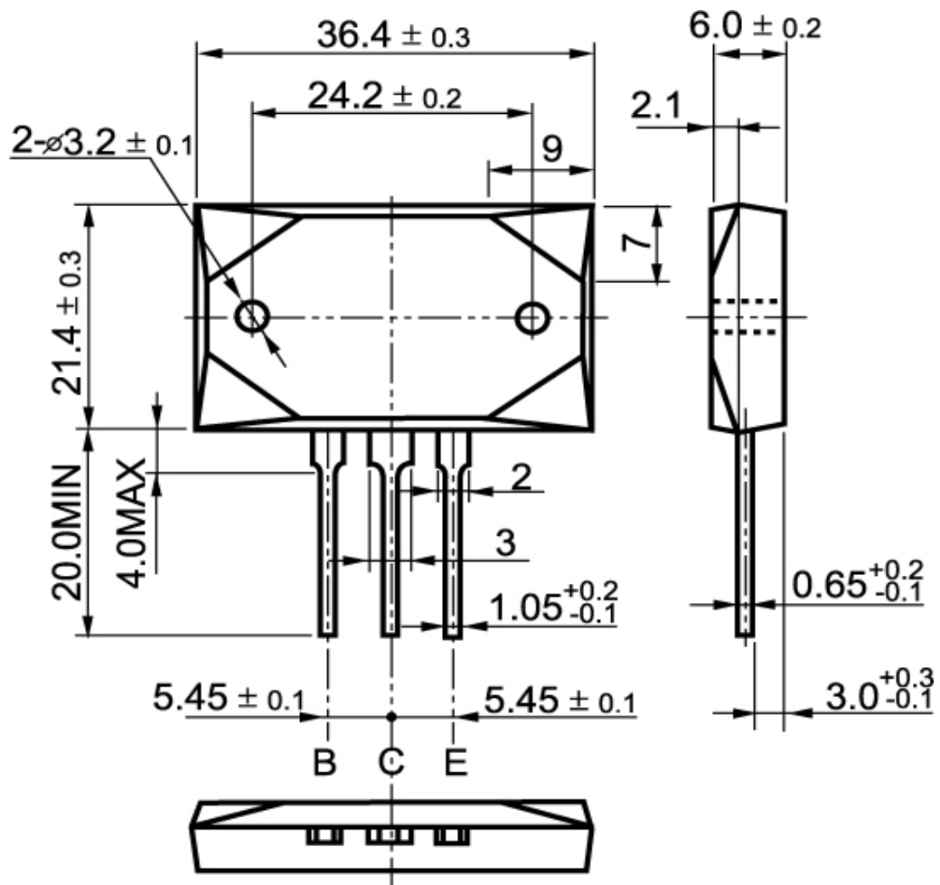
Fig.2 Outline dimensions
