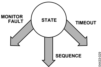
Figure 26. State Cell
