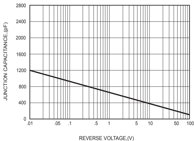
FIG.5-TYPICAL JUNCTION CAPACITANCE
