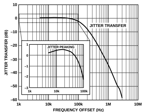
Figure 5. Jitter Transfer and Jitter Peaking
