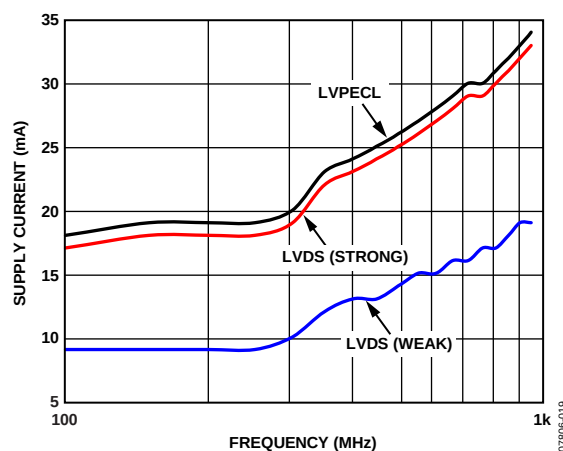
Figure 8. Supply Current vs. Output Frequency, LVPECL and LVDS (15 pF Load)
