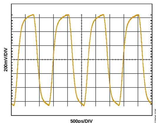
Figure 14. Typical Output Waveform, LVPECL (805 MHz)
