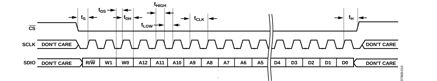
Figure 26. Serial Control Port Write—MSB First, 16-Bit Instruction, Timing Measurements
