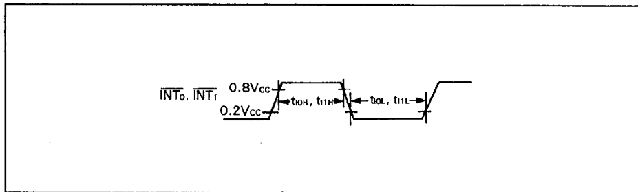
Figure 38. Interrupt Timing
