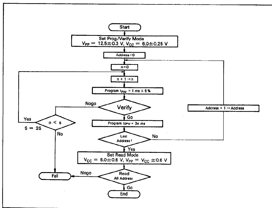
Figure 24. PROM Programming
