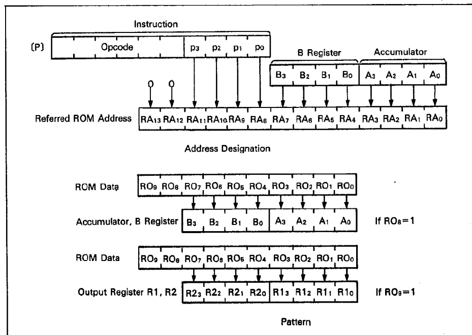
Figure 29. P Instruction
