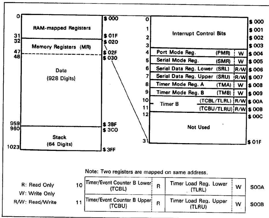
Figure 2. RAM Memory Map
