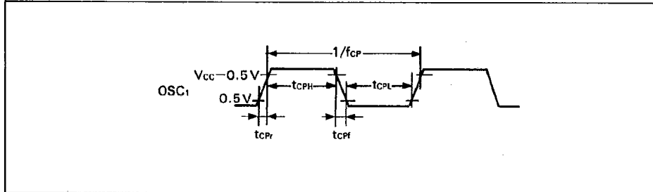
Figure 37. Oscillator Timing
