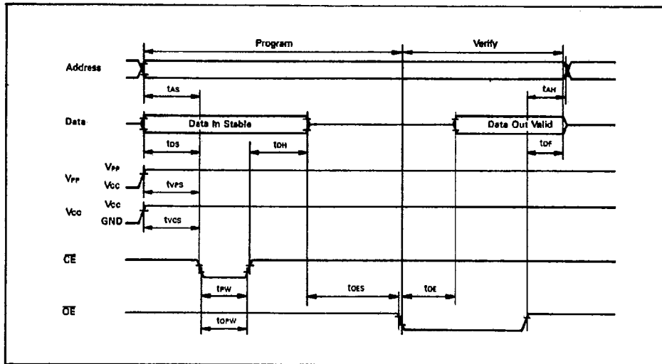
Figure 42. PROM Programming/Verify Timing
