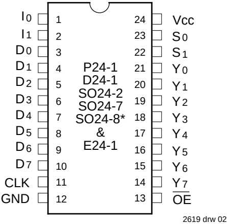
DIP/SSOP/SSOP/SSOP/CERPACK TOP VIEW
