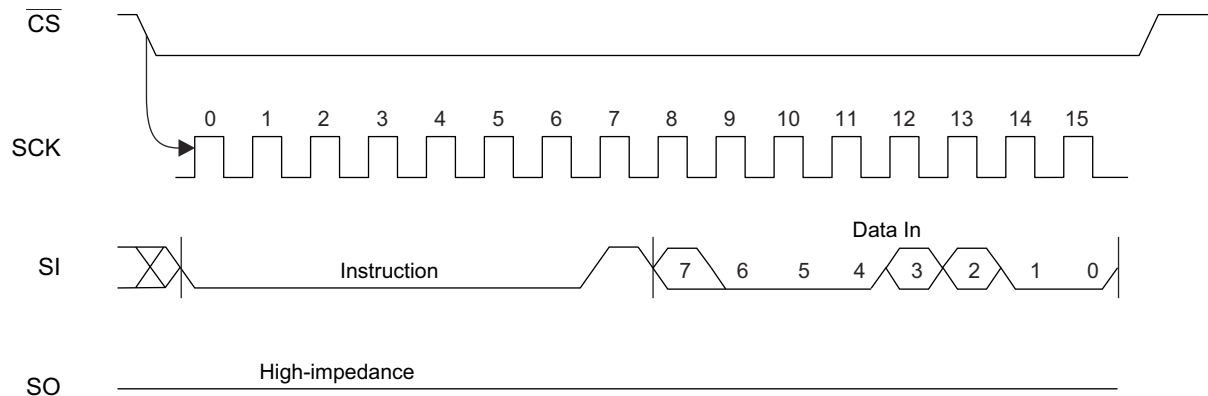
Figure 7-5. WRSR Timing
