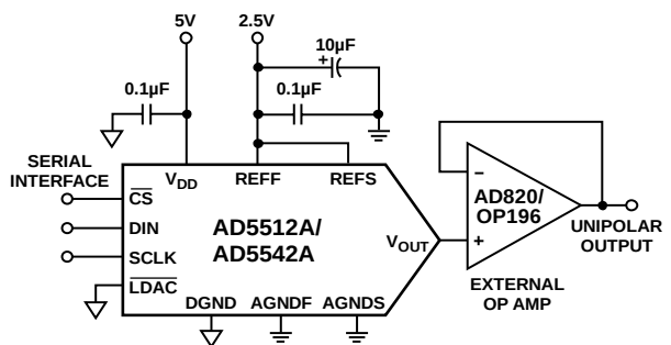
Figure 31. Unipolar Output
